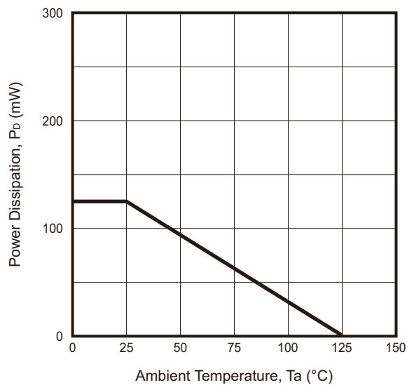
Fig.2 - Derating Curve
